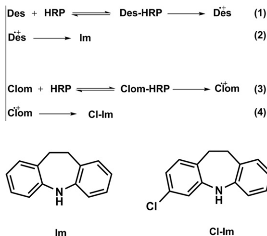
Figure 3. Reaction scheme of the drug's oxidation in the presence of HRP and \text{H}_2\text{O}_2 and the structures of the products. Des—desipramine, Im—iminodibenzyl, Clom—clomipramine and Cl-Im—3-chloroiminodibenzyl.
