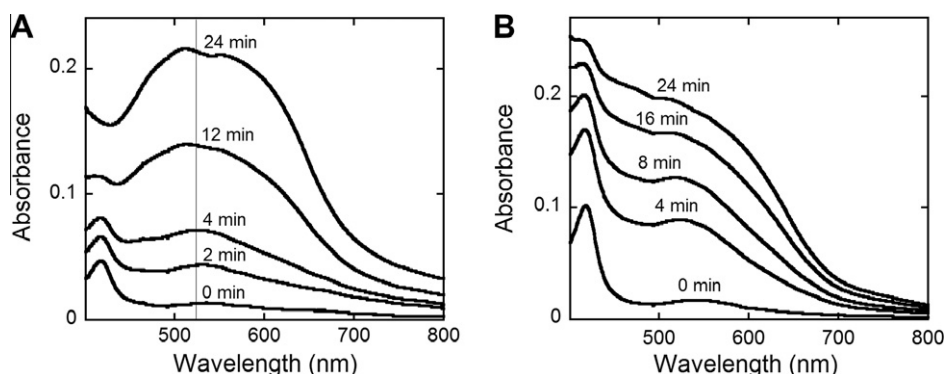
Figure 2. UV/vis absorption spectra of the drug's reactive intermediate formed during the oxidation by the HRP/ \text{H}_2\text{O}_2 system. (A) Reaction with desipramine performed in 133 mM Sorenson buffer pH 7.0. [HRP] = 0.6 \mu\text{M} ; [ \text{H}_2\text{O}_2 ] = 10 mM; [Desipramine] = 92 \mu\text{M} . (B) Reaction with clomipramine performed in water. [HRP] = 1 \mu\text{M} ; [ \text{H}_2\text{O}_2 ] = 10 mM; [Clomipramine] = 1 mM. The indicated times were when data were taken after the reagents were mixed.
