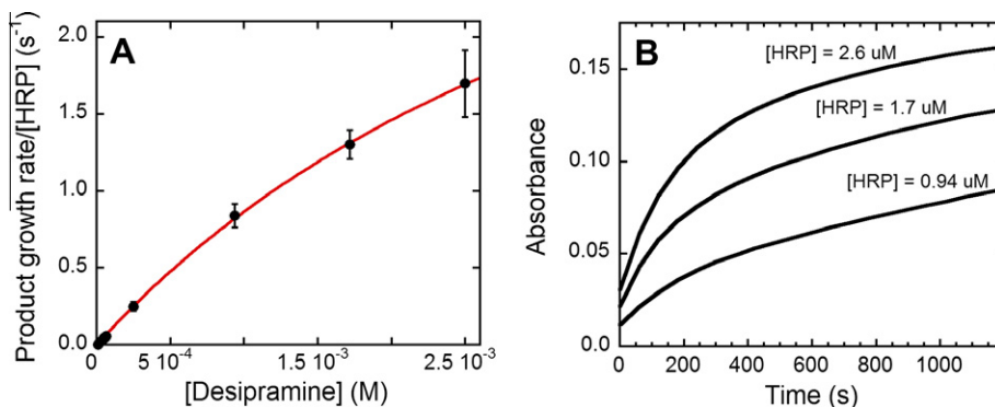
Figure 6. The kinetics of the formation of the desipramine radical monitored by UV/vis spectroscopy at 523 nm. (A) The initial slope (dA/dt) normalized by the extinction coefficient of the radical and the concentration of HRP, 0.498 \mu\text{M} , plotted against the concentration of desipramine. The error bars are standard deviations determined based on the 6–8 measurements of the absorbance growth rate and combined with the standard deviation of the extinction coefficient of desipramine radical. The red line represents the best fit curve obtained with Eq. (3). (B) The kinetics of the oxidation reactions of desipramine in the presence of HRP and \text{H}_2\text{O}_2 recorded for 20 min. [Desipramine] = 47 \mu\text{M} , [ \text{H}_2\text{O}_2 ] = 10 mM. The concentration of HRP for each curve is shown.
